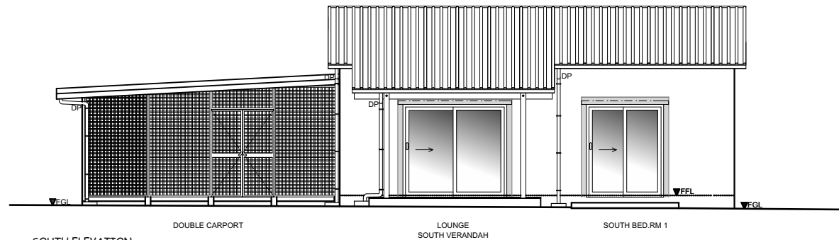
SOUTH ELEVATION
