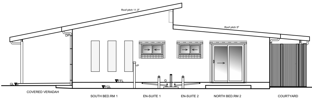
EAST ELEVATION
