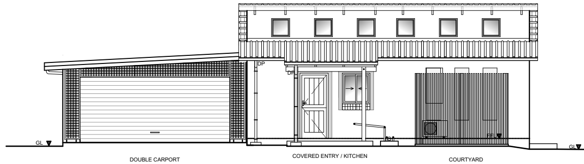
NORTH ELEVATION
