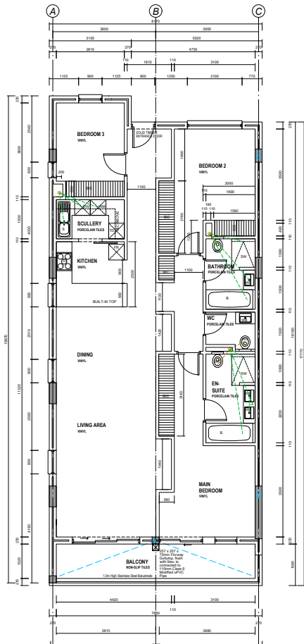
DETAIL LAYOUT UNIT TYPE A_scale 1:50 133m²; 2 per storey; Total: 8
