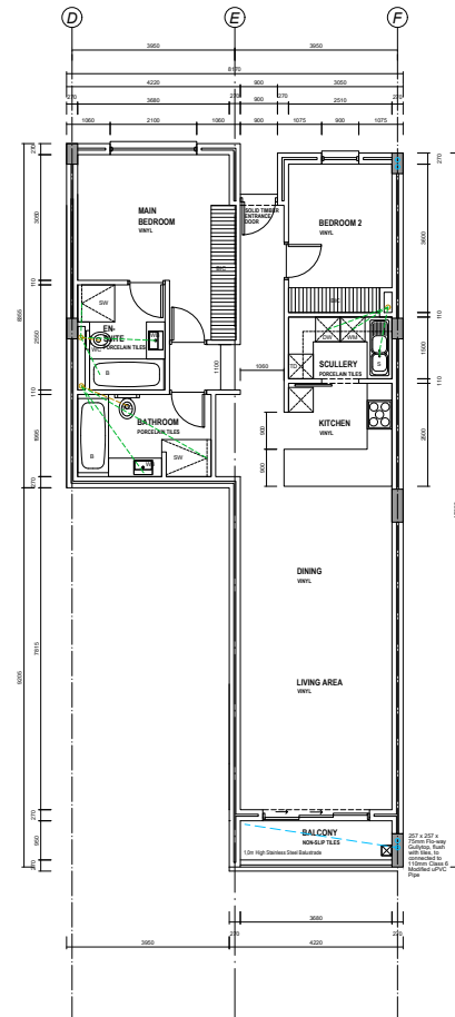
DETAIL LAYOUT UNIT TYPE C_scale 1:50 95m²; 4 per storey; Total 16
