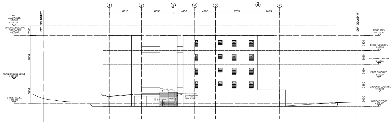
NORTH ELEVATION_scale 1:100
