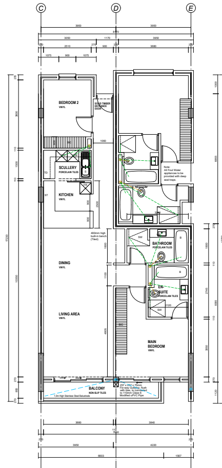
DETAIL LAYOUT UNIT TYPE B_scale 1:50 95m²; 4 per storey; Total: 16
