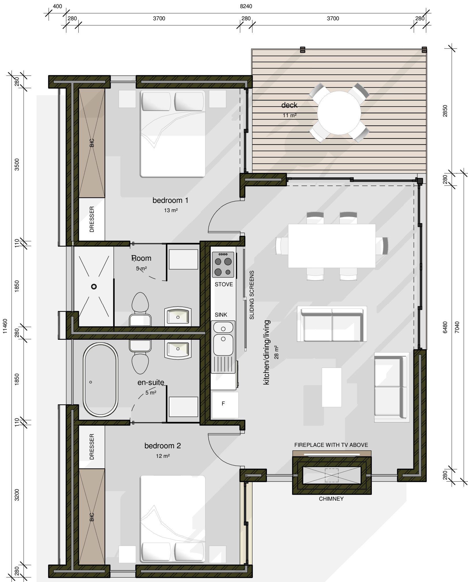
PLAN MULTI-BED UNIT : OPTION 1 (63m 2 + 11m 2 deck)
