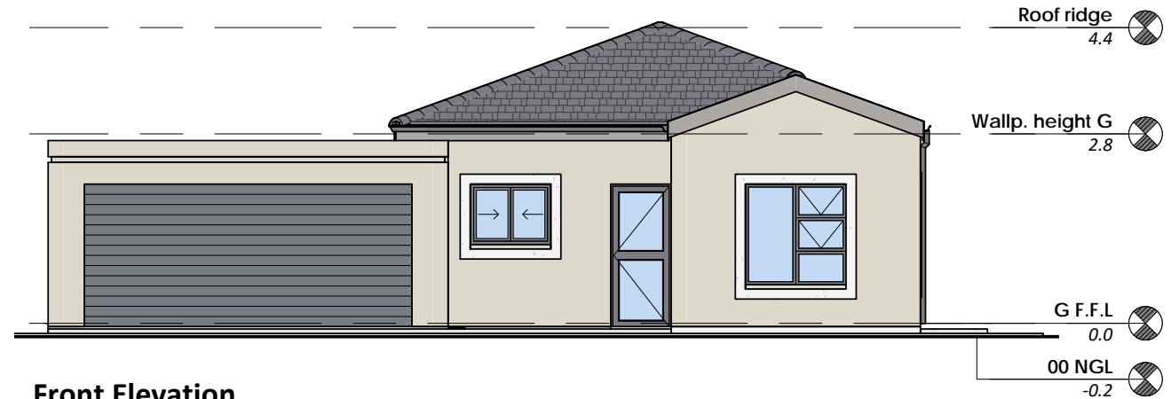
Front Elevation
