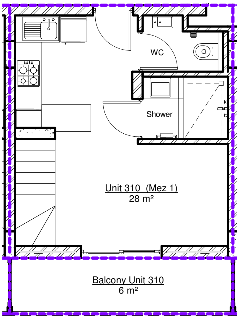
1 Unit 310 Lower Level 1 : 50
