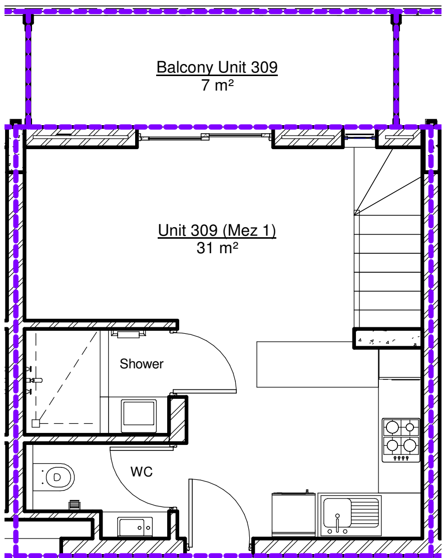
1 Unit 309 Lower Level 1 : 50
