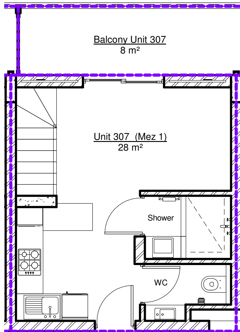
1 Unit 307 Lower Level 1 : 50
