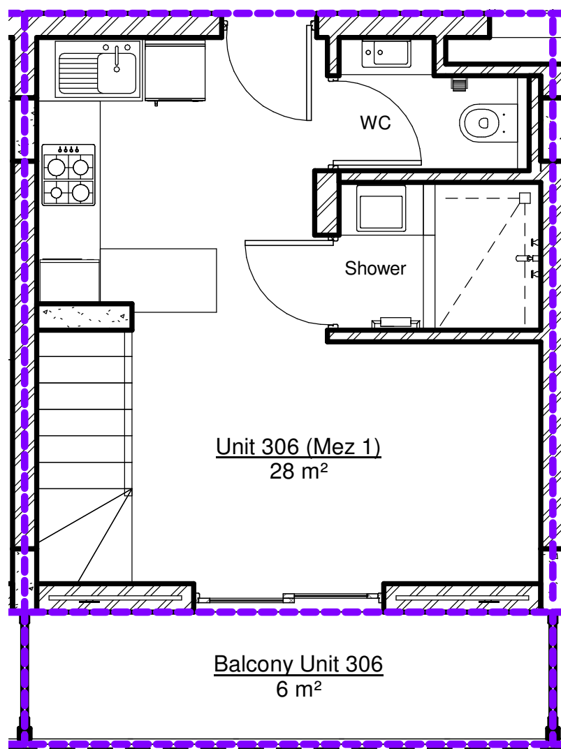
1 Unit 306 Lower Level 1 : 50
