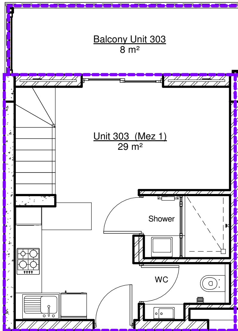
1 Unit 303 Lower Level 1 : 50
